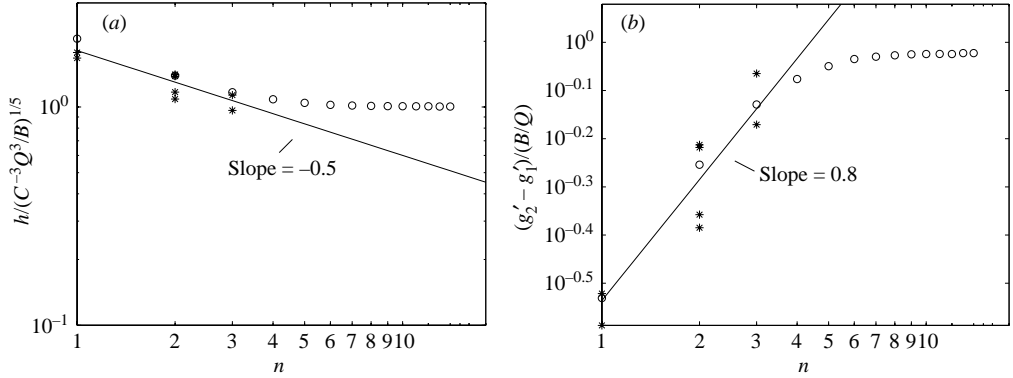
FIGURE 6. (a) The dimensionless interface height h/(C^{-3}Q^3/B)^{1/5} and (b) the non-dimensional density difference between two layers \hat{g}'_2/(B/Q) - \hat{g}'_1/(B/Q) plotted against the number of diffusers n when the total ventilation rate is fixed. The stars are the experimental results and the open circles are the results from the model.
