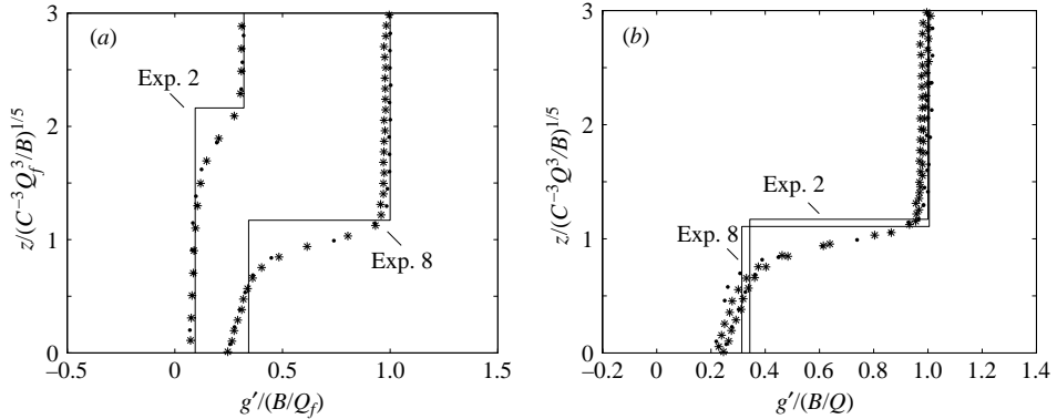
FIGURE 4. Dimensionless buoyancy profiles obtained at steady state with multiple diffusers for fixed heat load and underfloor pressure; Exp. 2 with 2 diffusers and Exp. 8 with 3 diffusers. (a) The buoyancy non-dimensionalized with the volume flux Q_f from each diffuser. (b) The buoyancy non-dimensionalized with the total ventilation volume flux Q .
