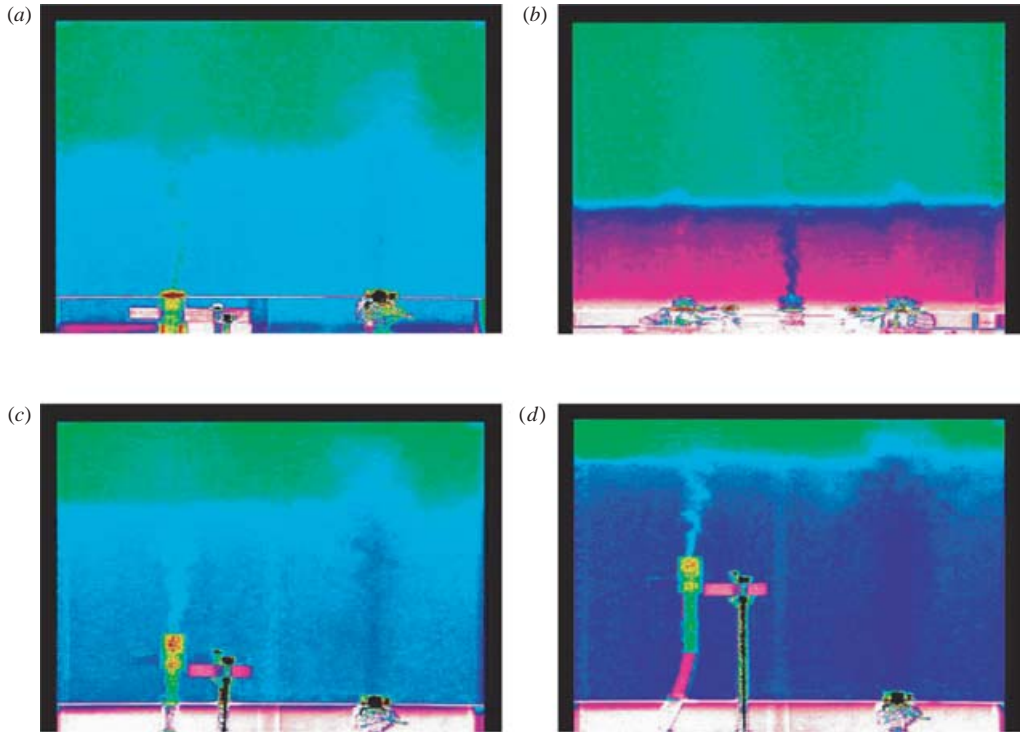
FIGURE 1. False colour images of the laboratory experiments in which water is used as the working fluid and saline and fresh water plumes and jets are used to represent thermal plumes and the flow from a cooling diffuser. The images have been inverted to represent the orientation appropriate to building ventilation (§3). (a) The basic case of one heat source and a single diffuser. (b) One heat source and two diffusers. (c) An elevated heat source at H/4 . (d) An elevated heat source at H/2 . In (c) and (d), the plume nozzle was fixed in the tank by a supporting bar. The effect of additional diffusers, for a given total flow rate, is to reduce the interface height and reduce the lower-layer temperature, while raising the heat source above the floor raises the interface and reduces the lower layer temperature.
