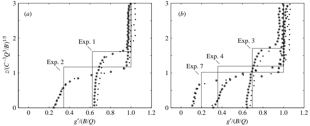
FIGURE 3. Buoyancy profiles obtained at steady state with multiple diffusers with fixed heat load and ventilation rate. The height is made dimensionless by the height scale C^{-3/5}Q^{3/5}B^{-1/5} based on the total ventilation rate and buoyancy flux, and the buoyancy by the buoyancy scale B/Q . (a) Exp. 1 with a single diffuser and Exp. 2 with two diffusers; (b) Exp. 3 with one diffuser, Exp. 4 with two diffusers and Exp. 7 with three diffusers.
